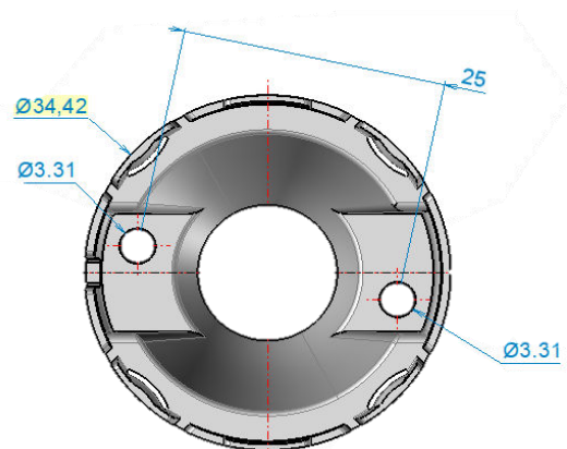
Collimator with holder
