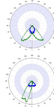
POLLUX7X1DA35 Double Asymmetric
