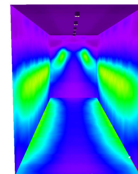
POLLUX7X1DA35 Double Asymmetric
